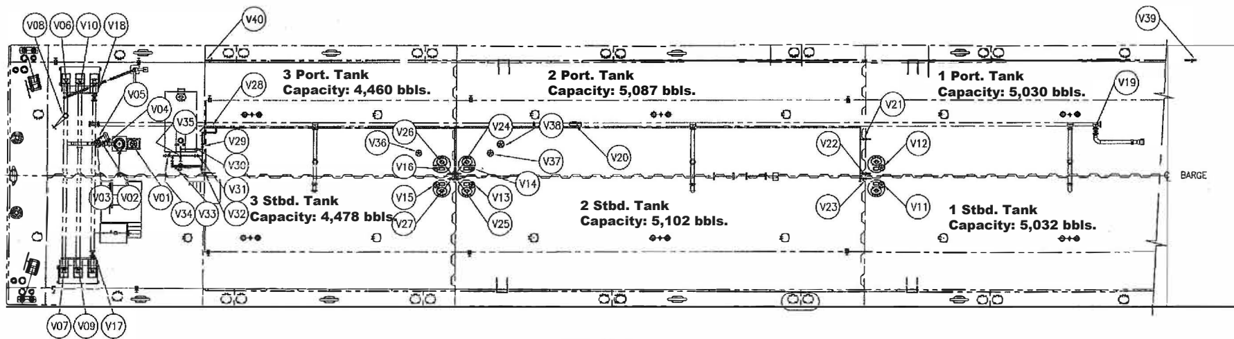
DECK PLAN
