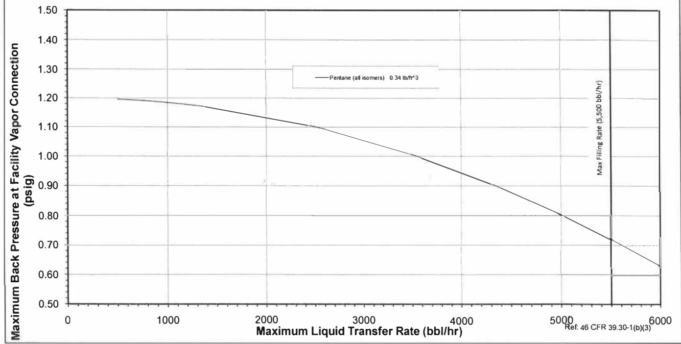
Curve of Allowable Back Pressure at Facility Connection
